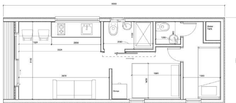
Layout 4: 9m x 3.5m x 3.5m with Bunk Beds
